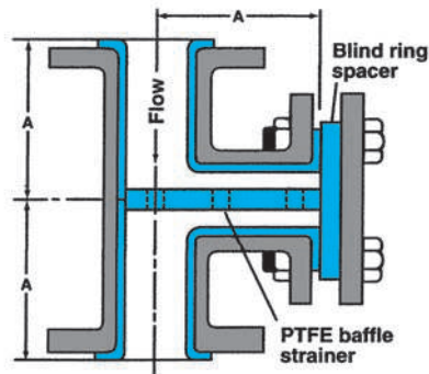
Strainer Tee
