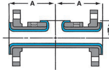
Short Stack Tee (tapped holes straddle C i )
