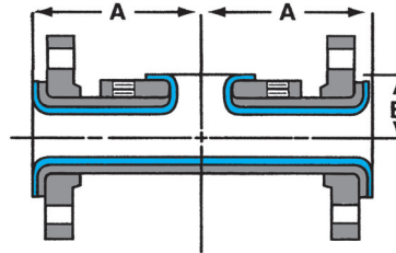
Short Stack Tee (tapped holes straddle C L )
