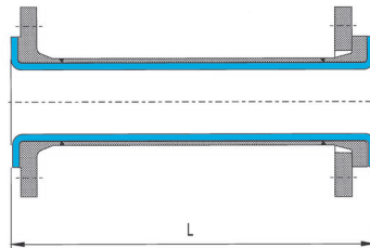
fixed - loose
