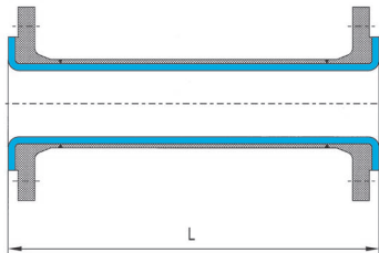
fixed - fixed
