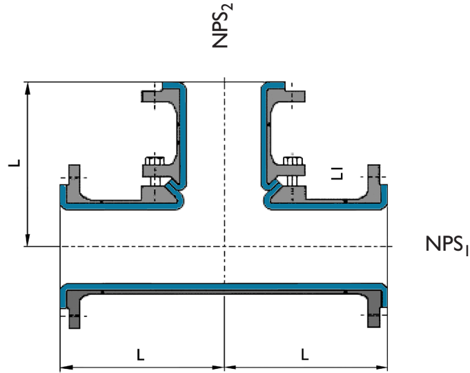
(6"-12" PTFE) (two-piece design)
